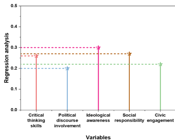
Figure 4. Result of regression analysis.
