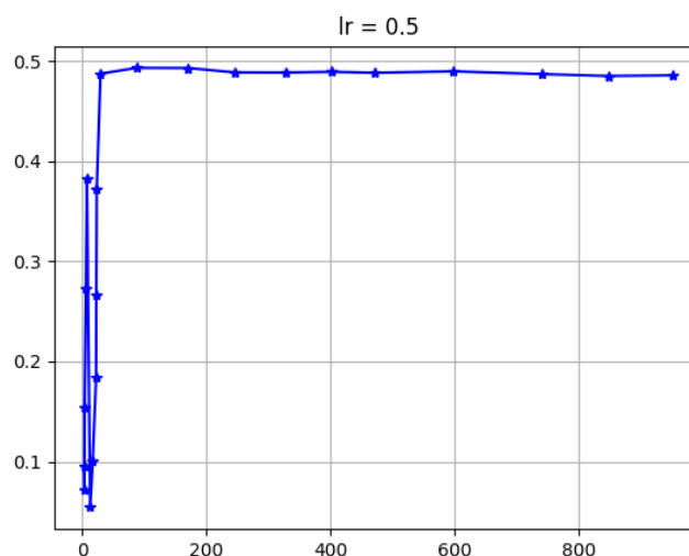
Figure 8. Error change chart when learning rate is 0.5.
