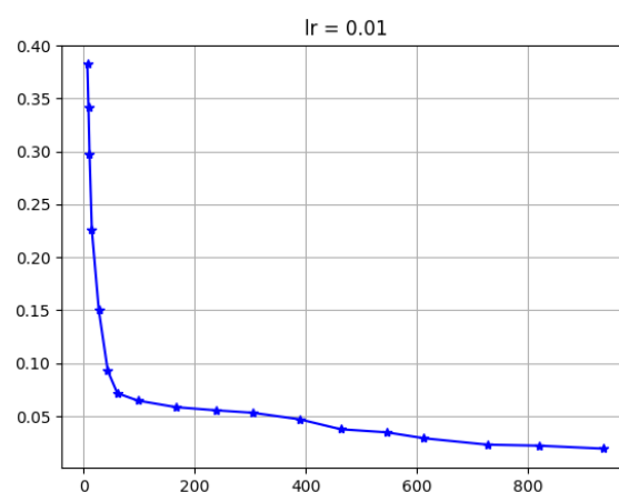
Figure 10. Error change chart when the learning rate is 0.01.
