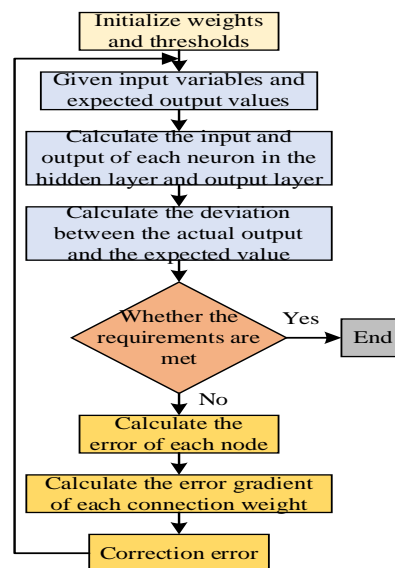
Figure 4. Working mechanism of BP neural network.
