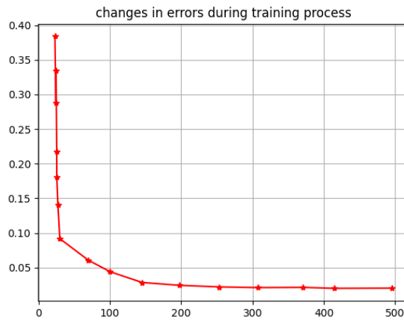
Figure 11. Error change chart of model training.
