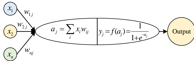
Figure 3. Working mechanism of neurons.
