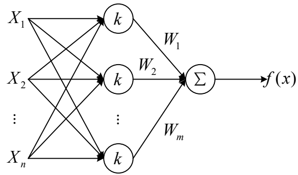
Figure 5. RBF network structure.
