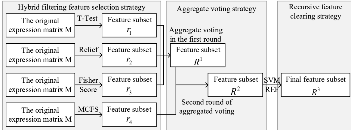
Figure 1. Frame diagram of FVR feature selection algorithm multi-strategy approach.
